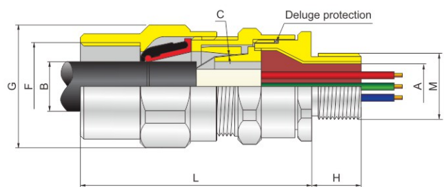
Steel pipe wiring DQM-III/II-G
