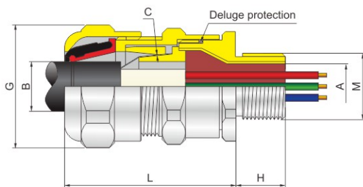
Cable wiring DQM-III/II-D
