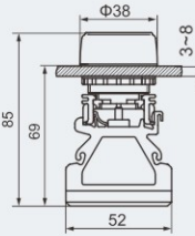
Control button cover mounting
