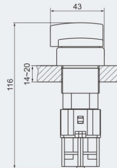
Three-position switch
