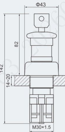
Key-operated mushroom emergency push button
