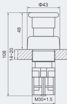
Mushroom stay-put/ turn-to-release emergency push button
