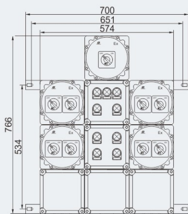
BXM(D)53-8/□/K/□
