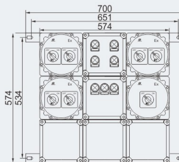
BXM(D)53-6/□/K/□
