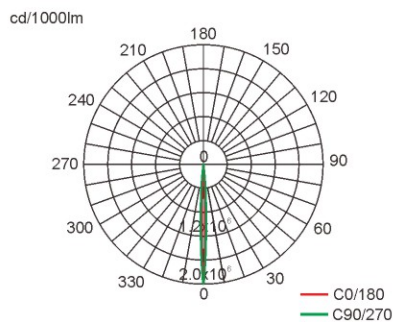
配光曲线 Light distribution curve
