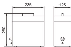
电池箱 Battery Box
