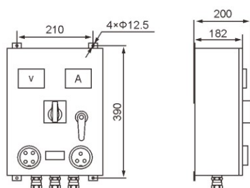
CXD8-CDX 充电箱 Charger Box
