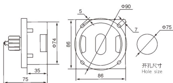
CXZ8-1 插座(室内) Socket (indoor)
