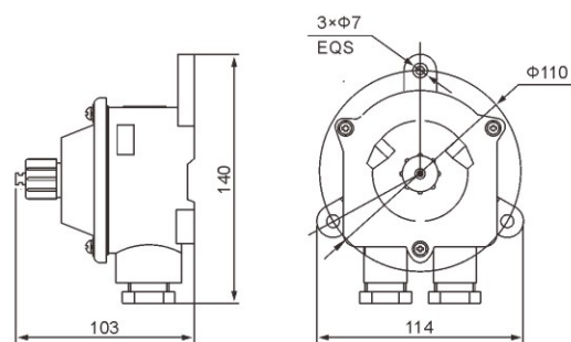
CXZ8 插座(室外) Socket (outdoor)
