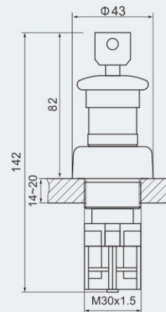
Key-operated mushroom emergency push button
