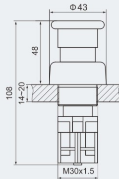
Mushroom stay-put/ turn-to-release emergency push button
