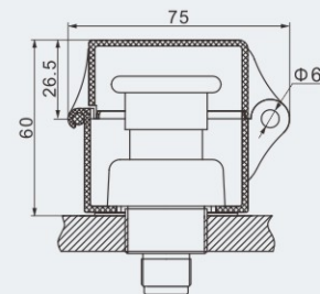
HA Emergency push button with PC protection cover
