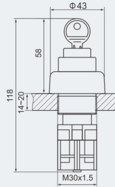
Key-operated push button
