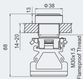
Push button with indicator
